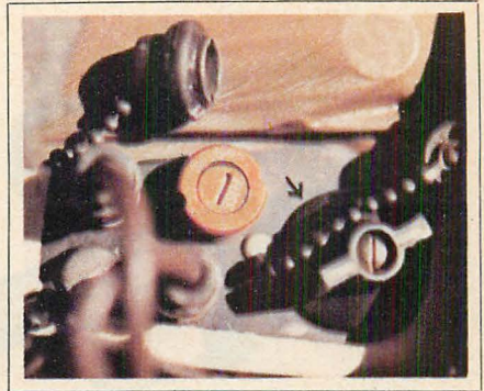
Close-up of power-pack on typical infrared device. Is mounted in backpack assembly with 6-volt power source. Knob at lower right (see arrow) is off-on switch. Output cables to both IR light source and electronic telescope are located at lower left. Manipulation of switch is made easy by location in opening in bottom of backpack.
